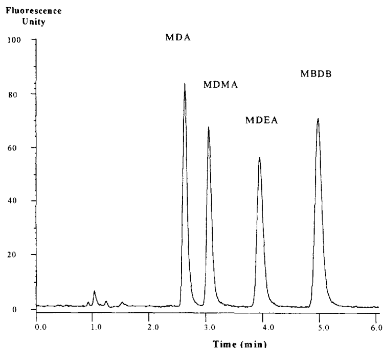
Fig. 2. Separation of four methylenedioxyated amphetamines by HPLC on a Macherey-Nagel column (125×4 mm) C 18 AB Nucleosil 100 (5 μm); mobile phase: NaH 2 PO 4 solution (adjusted to pH 3.8)–acetonitrile (85:15); flow-rate: 1 ml min -1 ; fluorimetric detection set at Ex: 285 nm, Em: 320 nm.
