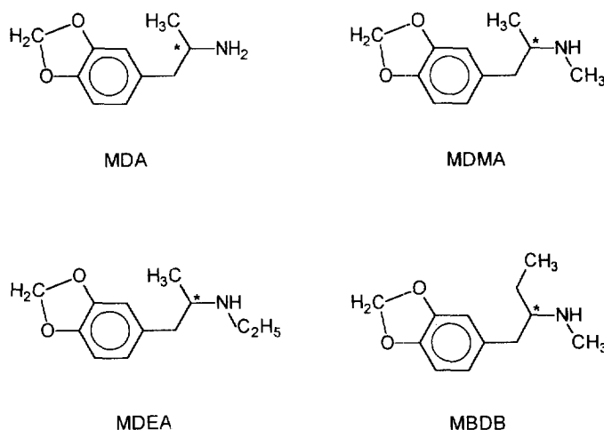
Fig. 1. Chemical structure of the analyzed methylenedioxyated amphetamines.
