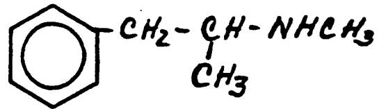
Methamphetamine
