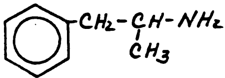
Amphetamine
