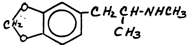
MDMA
