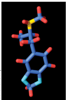
MDMA
