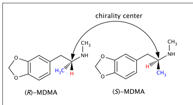
Figure 1: Chemical Structure of MDMA
